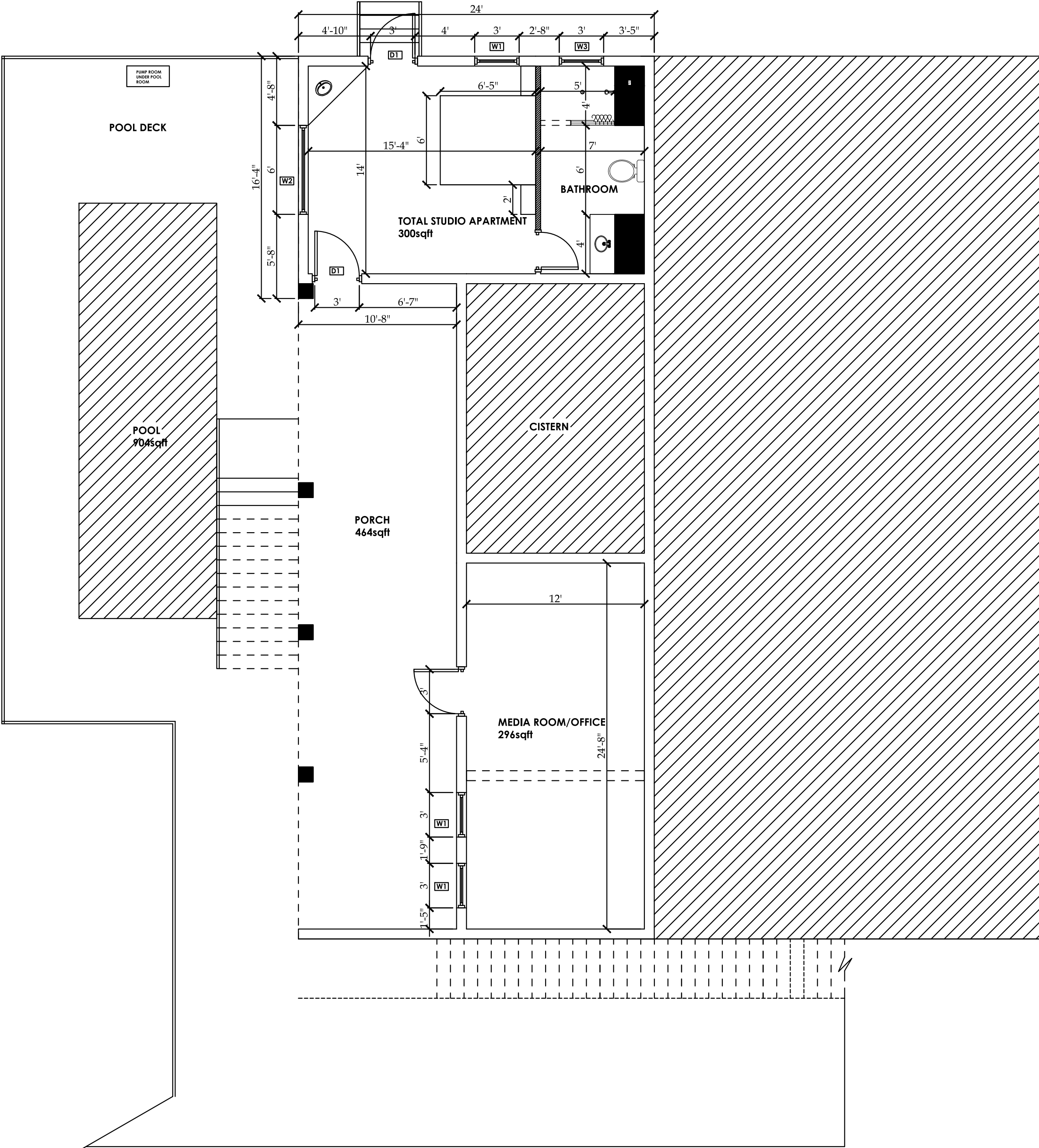
GROUND FLOOR PLAN 2328 tot. sqft
